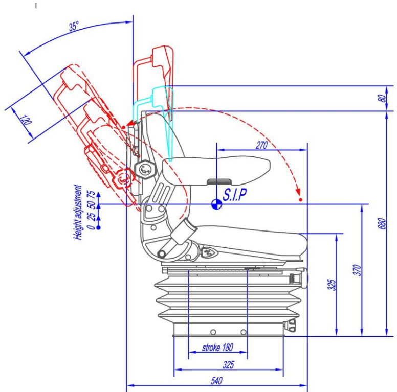
SUSPENSION MECANIQUE
