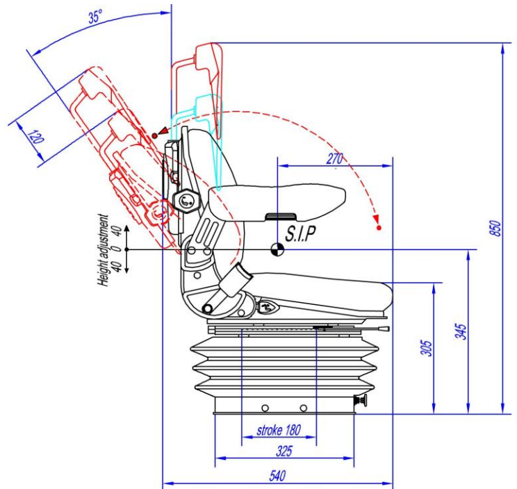
SUSPENSION MECANIQUE
